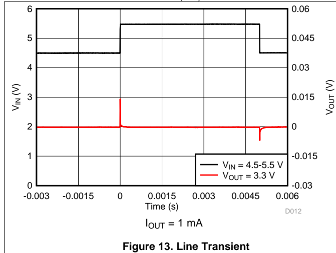
Figure 13. Line Transient
